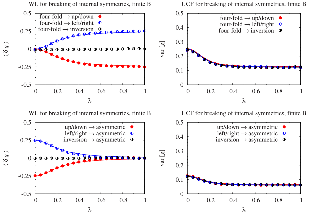
FIG. 9. (Color online) Same as Fig. 8, but for a finite magnetic field.
