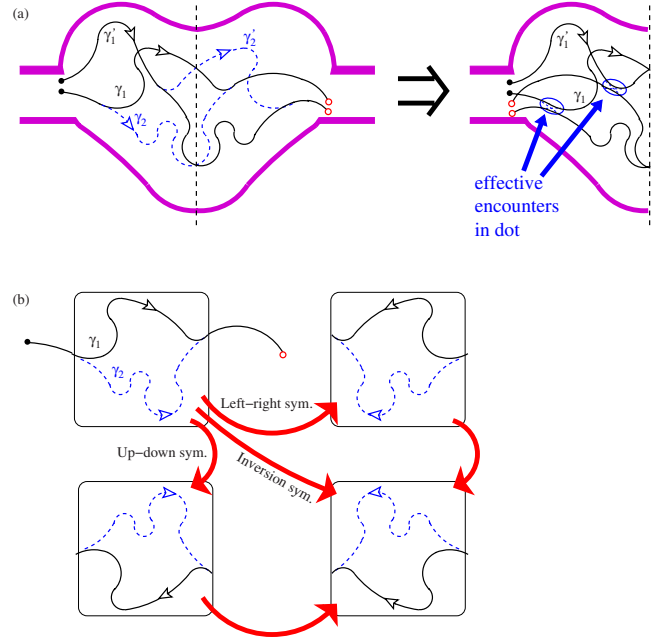
FIG. 6. (Color online) (a) A contribution to universal conductance fluctuations in a left-right mirror-symmetric system. On the right we show the same contribution folded into half the dot, such that one can see the two effective encounters (we only show the dashed paths at the encounters). (b) The full list of pairings for path \gamma_1 and \gamma_2 , with left-right, up-down and inversion symmetry. There are also contributions in which paths are paired with the time-reverse of their images (arrows reversed); indeed, (a) is an example of this for a left-right symmetric system.
