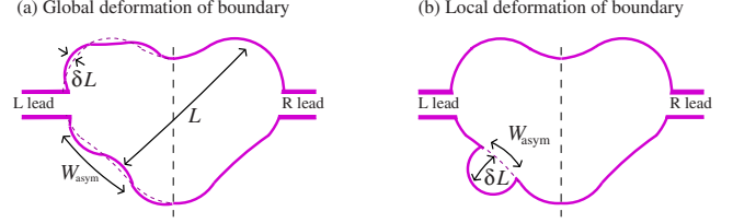
FIG. 3. (Color online) Two ways in which the left half of a quantum dot can be deformed away from symmetry with the right half. In (a), the left half is deformed over a long range W_{\text{asym}} \gg \lambda_F by a gentle ripple of small magnitude \delta L < \lambda_F . A special case of this is where the whole left half of the dot is deformed outwards by a distance of order \delta L , then W_{\text{asym}} \sim L . In (b), a small part of the boundary of the left half (of width W_{\text{asym}} ) is deformed by a distance \delta L \gg \lambda_F . In the former case, the parameter which controls the deviation from symmetry is \delta L/\lambda_F while in the latter case it is W_{\text{asym}}/L .
