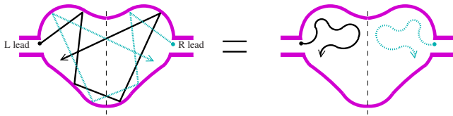
FIG. 1. (Color online) Sketch of a planar quantum dot with a left-right mirror symmetry. On the left we show a classical path (solid line) and its mirror image (dashed line). Each path is piecewise straight and undergoes specular reflections at the boundary of the dot. The path is chaotic (we assume hyperbolic chaos), so its position and momentum after time t are exponentially sensitive to the initial position and momentum. We assume the system is such that a typical path crosses the symmetry axis a large number of times before escaping into a lead (these crossings occur on a time scale of order of the time-of-flight across the system). To simplify the sketches elsewhere in this article, we draw paths as abstract curves (shown on the right) which only show those crossings of the symmetry axis that are crucial to the nature of the path.
