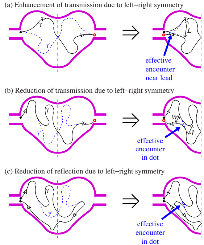
FIG. 2. (Color online) Contributions to weak localization due to a left-right mirror symmetry. When we fold the paths into one half of the dot (as shown in the right-hand sketches), paths hitting the symmetry axis are specularly reflected; however, we must keep track of whether the path escapes into the right lead. Thus, in those sketches, paths that end on the left lead are marked with solid circles, while those that end on the right lead are marked with open (red) circles. The sketch in (a) is an enhanced forward-scattering contribution, because it enhances transmission through the dot.
