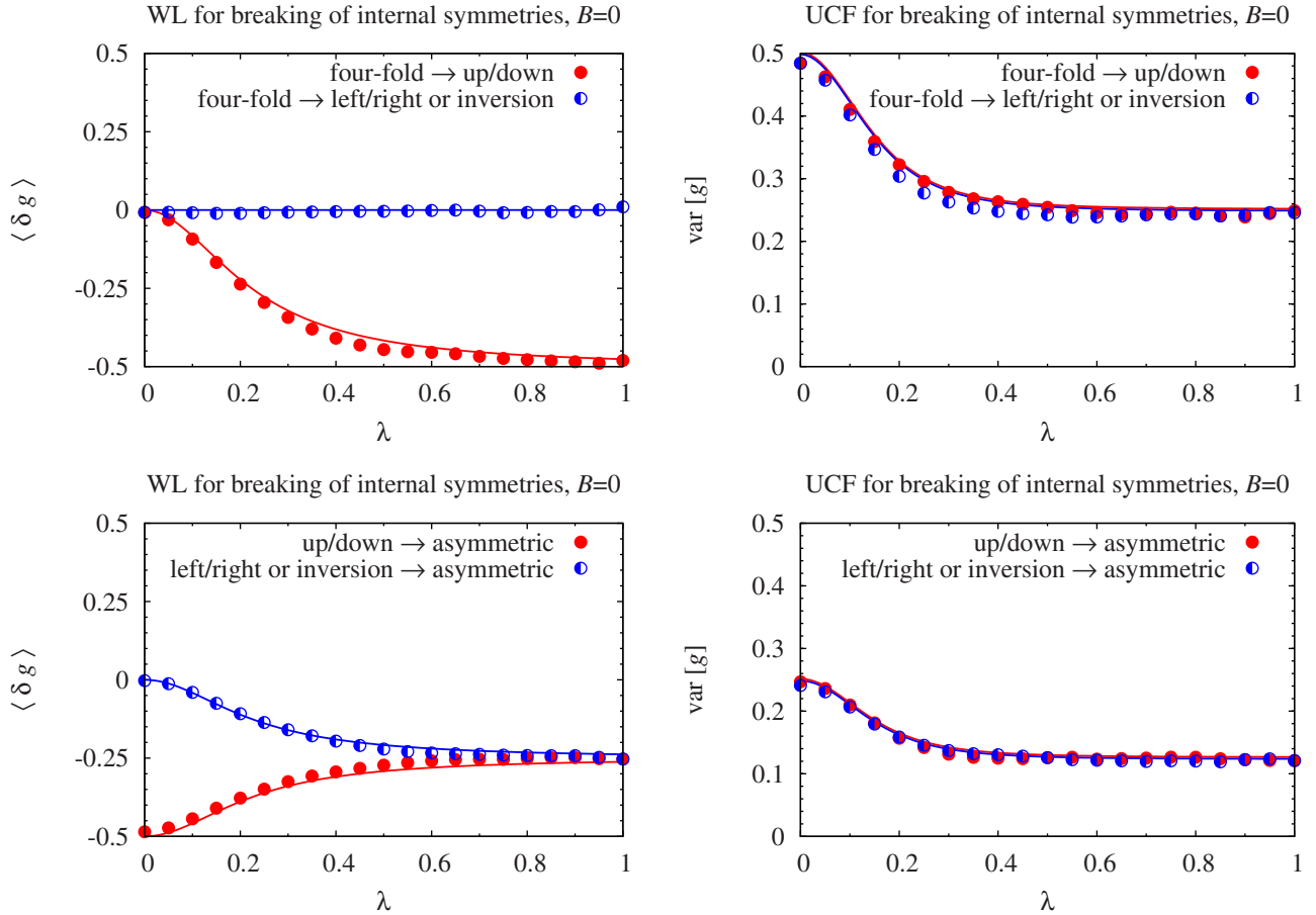
FIG. 8. (Color online) Same as Fig. 7, but for transitions induced by the breaking of internal spatial symmetries ( B=0 ).
