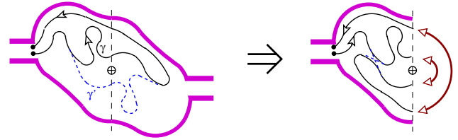
FIG. 4. (Color online) Contributions to weak localization due to an inversion symmetry, which is equivalent to symmetry under a 180^\circ rotation about the point indicated by \oplus . In the folded sketches on the right-hand side, paths that end on the left lead are marked with solid circles, while those that end on the right lead are marked with open (red) circles (as in Fig. 2). When we fold all paths into one half of the dot (see the right-hand sketches) by rotating the other half of the dot by 180^\circ , any path which crosses the line between the two halves (dashed line) at (r, p) reappears at (-r, -p) , where r=0 is defined as the center of the inversion symmetry (marked \oplus ). The sketch in (a) is an enhanced forward-scattering contribution similar to that in Fig. 2(a).
