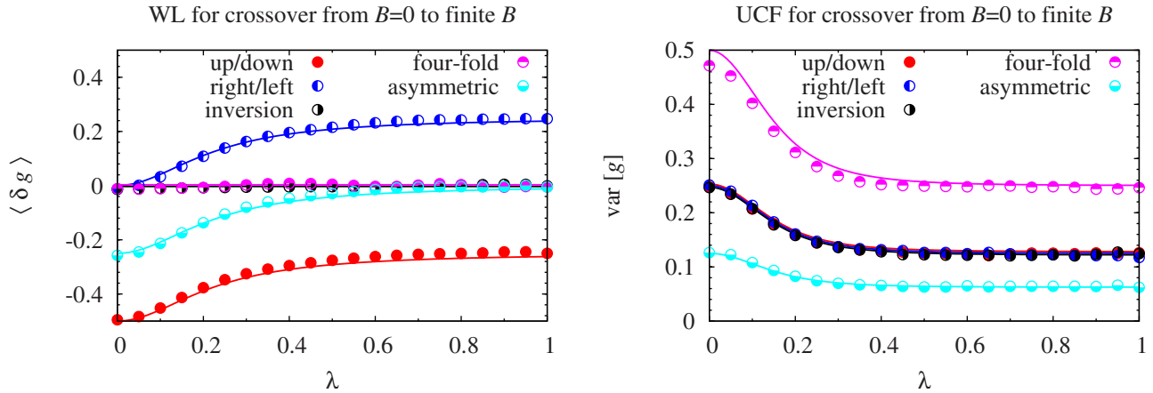
FIG. 7. (Color online) Effect of a magnetic field B=(\lambda/\lambda_c)B_c \approx \lambda B_0 on the weak-leak localization correction (left panels) and the conductance fluctuations (right panels) for quantum dots of different spatial symmetry. The solid lines show the universal crossover functions (46) and (47), derived in this paper based on semiclassical arguments. The data points show the result of numerical computations based on the interpolation formulas Eqs. (41) and (42) between the random-matrix ensembles tabulated in Table II. In these computations, M=1000 and N=50 , resulting in \lambda_c=1/\sqrt{20} . Each data point is obtained by averaging over 5000 realizations.
